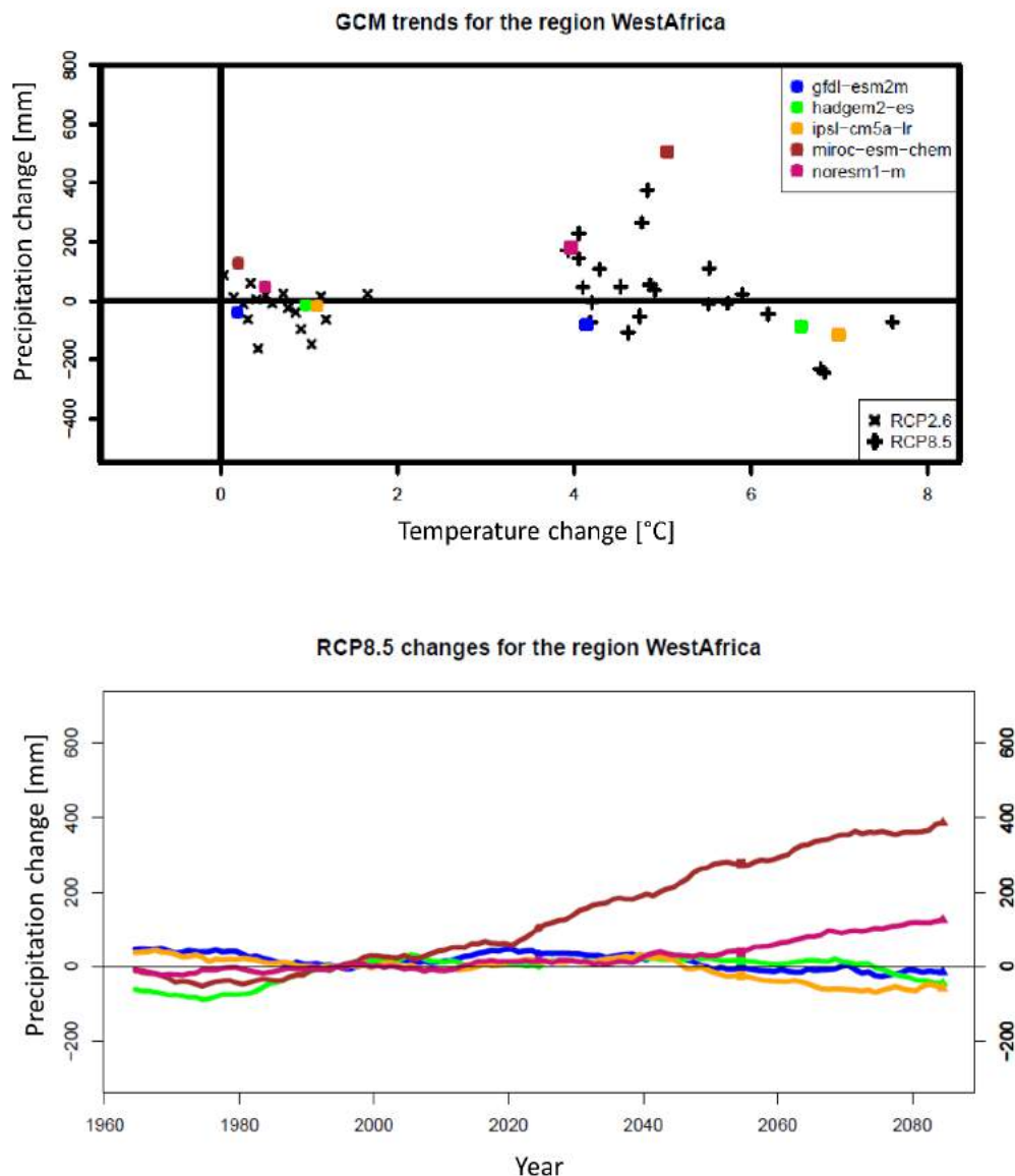
Figure 33: Model spread in temperature and precipitation change until the end of this century.
