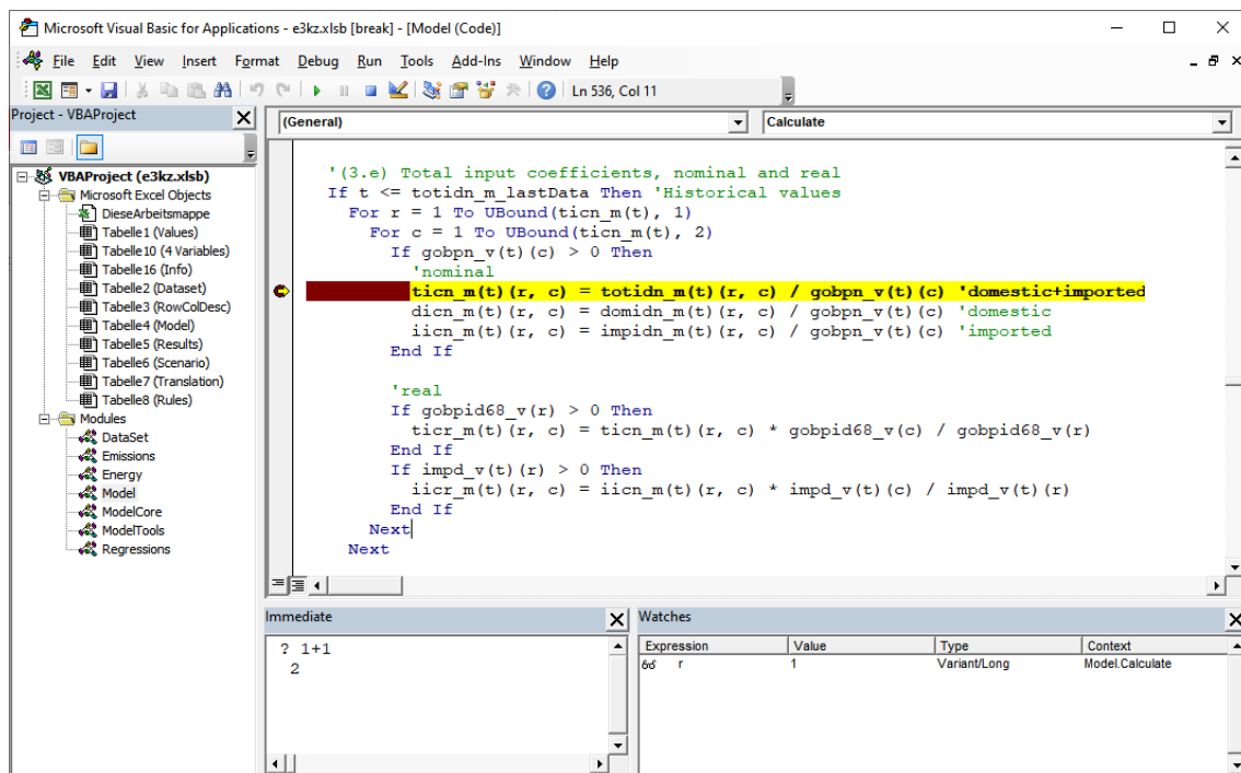
Figure 11: Model debugging
